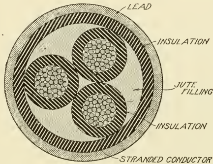
Fig. 50. Section of Polyphase Cable
